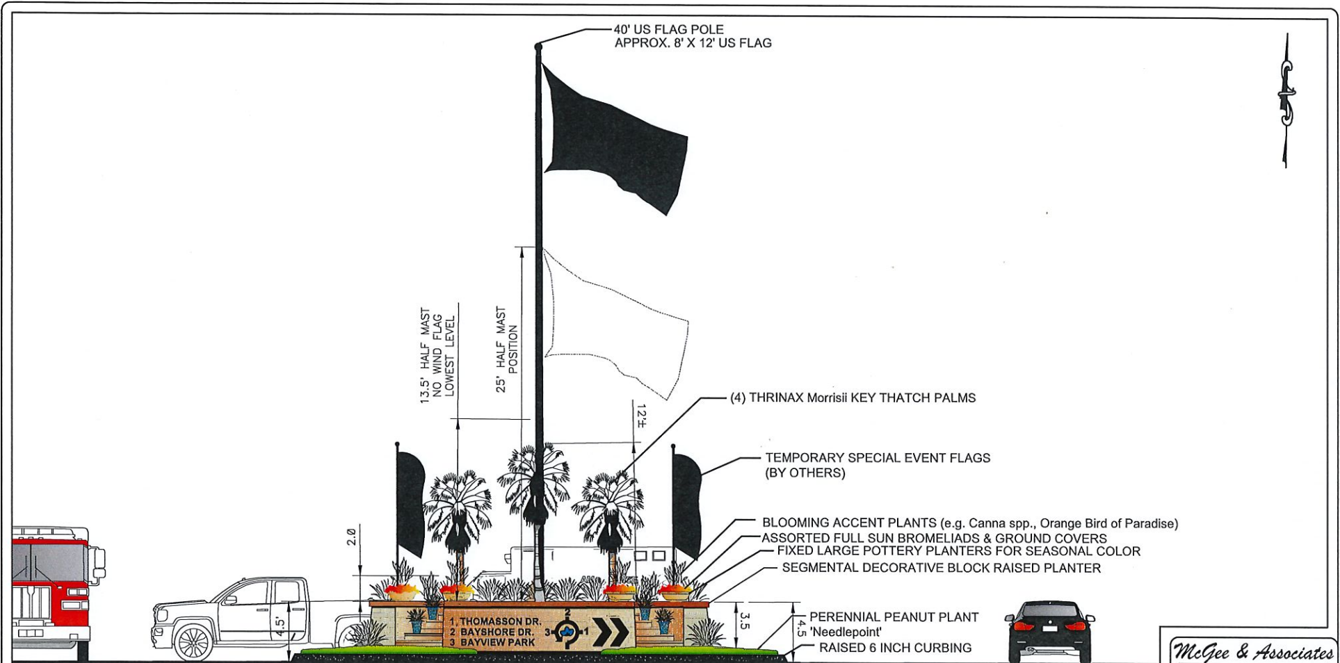
NORTH BOUND BAYSHORE DR. AT BOTANICAL GARDEN CONCEPTUAL SECTION / ELEVATION
